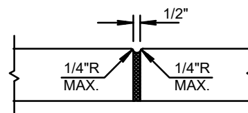
EXPANSION JOINT
