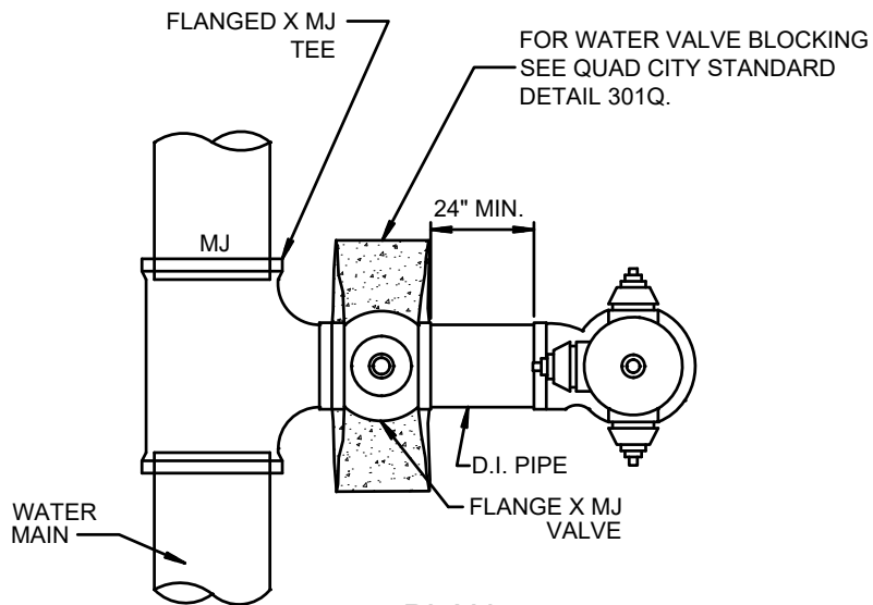
PLAN
