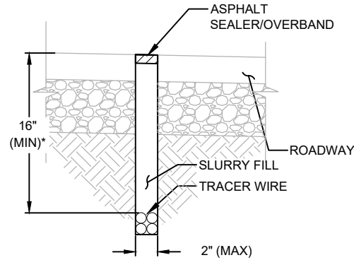
TRENCH TYPICAL INSTALLATION NOT TO SCALE
