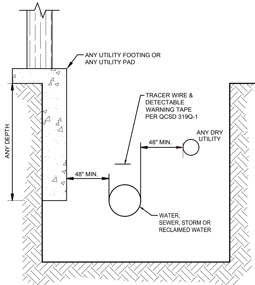
HORIZONTAL CLEARANCE
