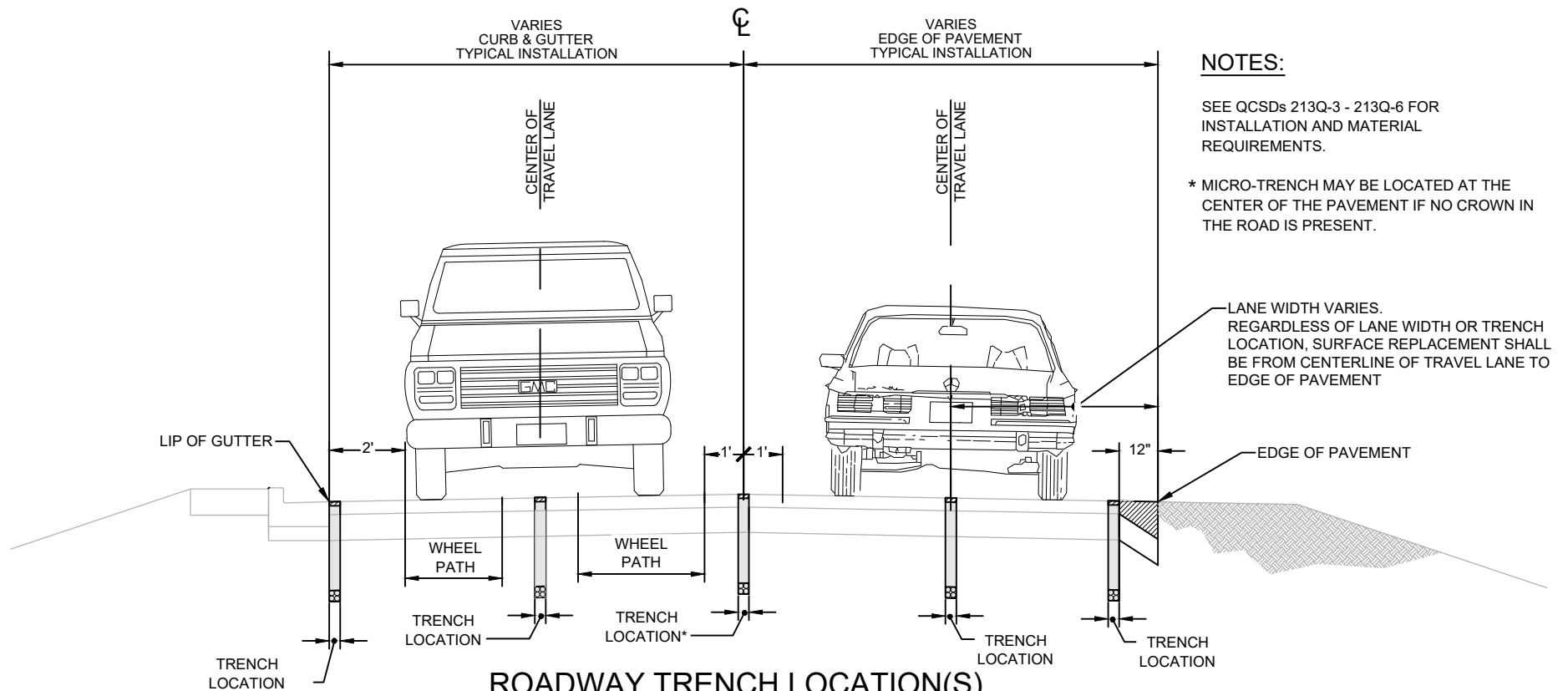
CURB & GUTTER TYPICAL INSTALLATION NOT TO SCALE
