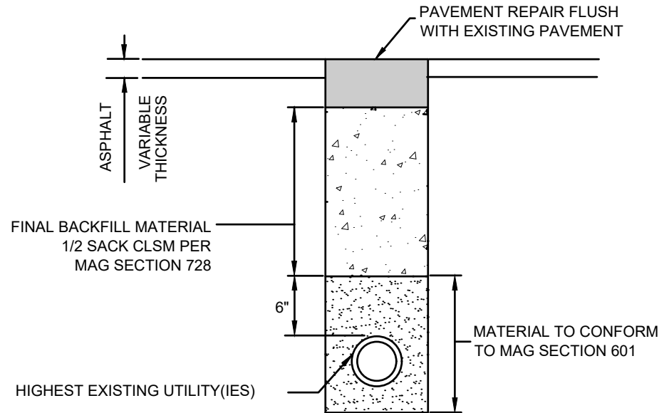
SECTION VIEW
