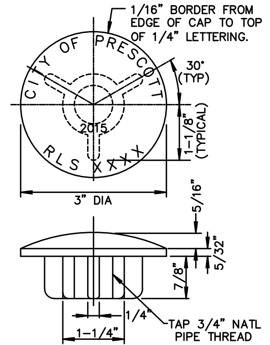
CAP DETAIL
